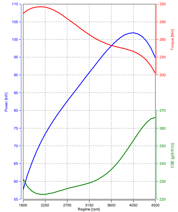
Performances curves
