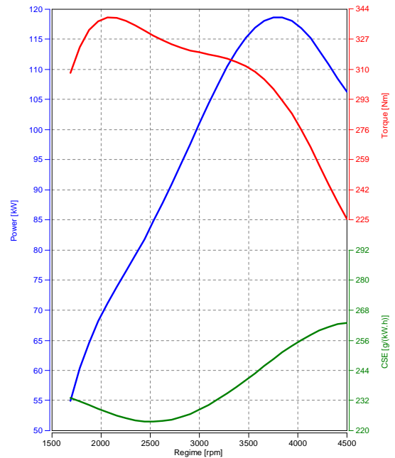
Performances curves
