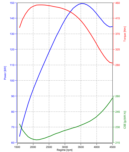
Performances curves
