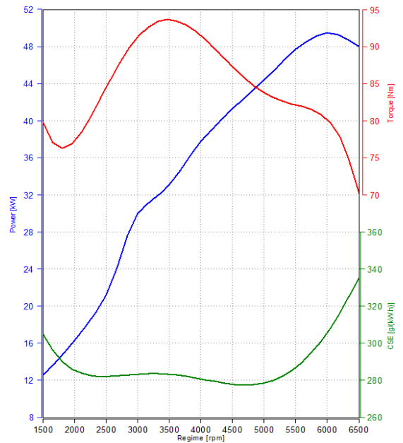
Performances curves
