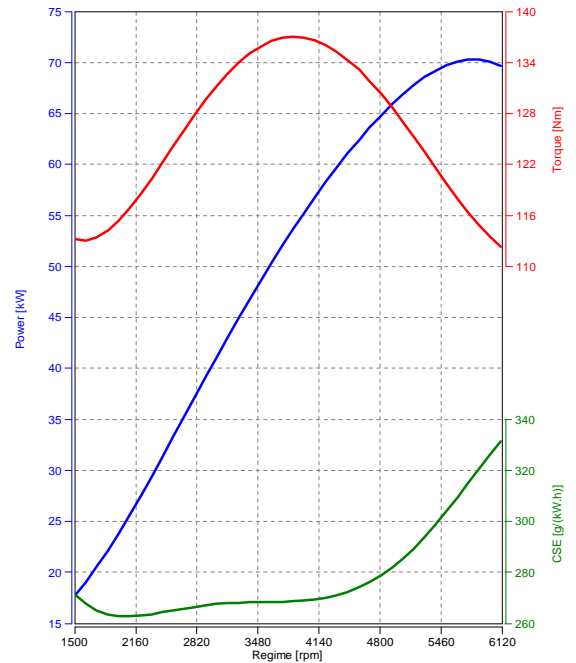
Performances curves
