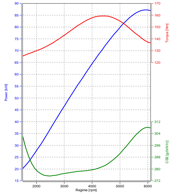
Performances curves
